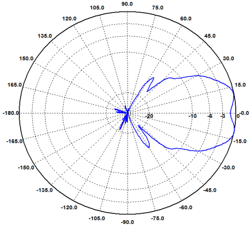
E-Ebene / E-Plane 13 GHz
