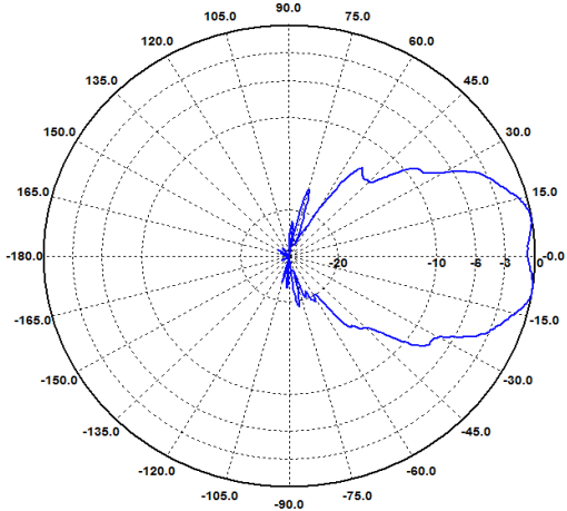
E-Ebene / E-Plane 14 GHz
