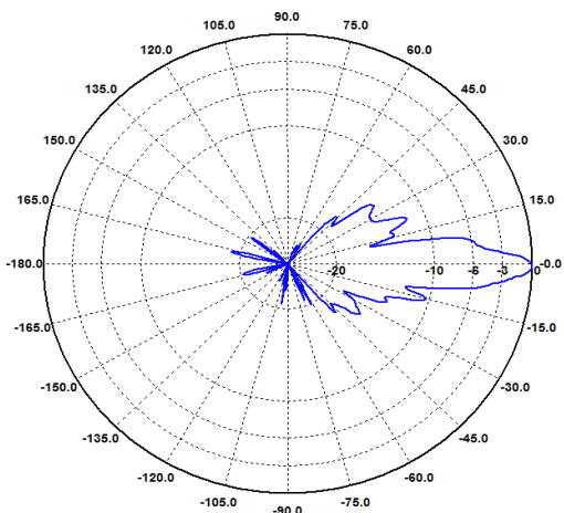
E-Ebene / E-Plane 18 GHz
