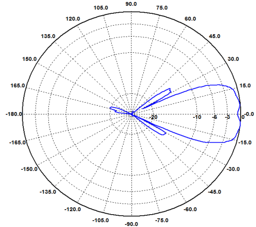
H-Ebene / H-Plane 13 GHz
