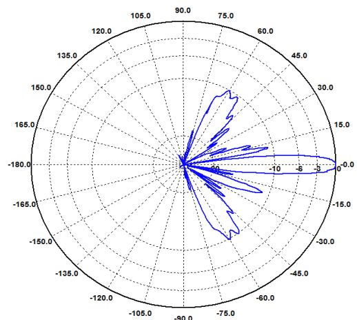
H-Ebene / H-Plane 18 GHz
