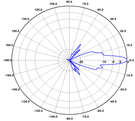
H-Ebene / H-Plane 17 GHz
