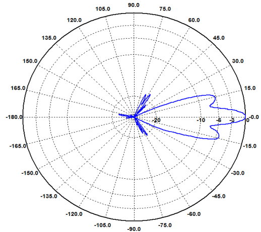
H-Ebene / H-Plane 16 GHz
