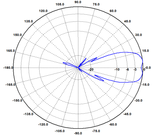
H-Ebene / H-Plane 14 GHz
