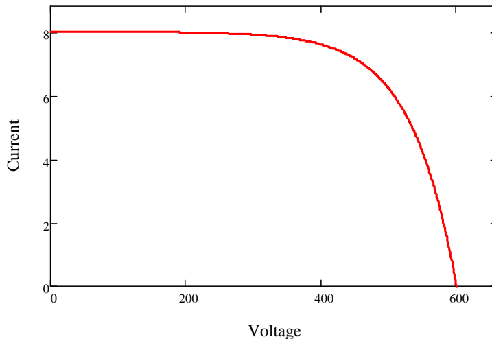
Current/voltage characteristic of real solar cells
