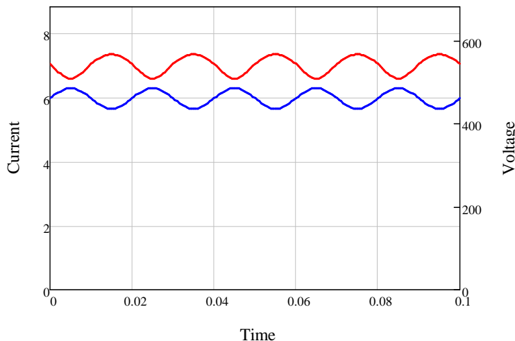
Phase shift between current and voltage at ripple 50Hz
