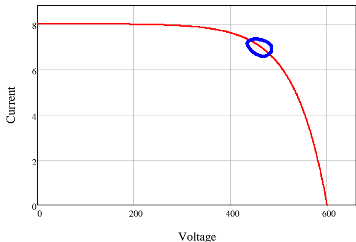
Operating points (blue) when using switch-mode simulator
