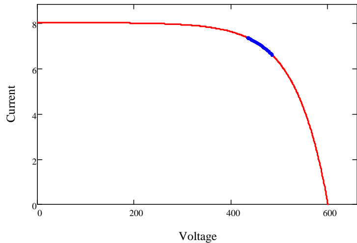
Operating points (blue) when using PVS
