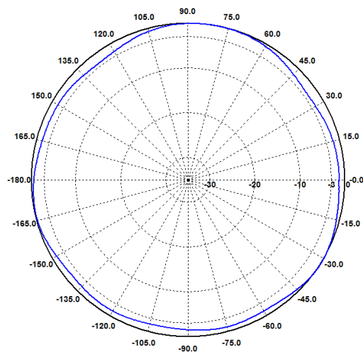
H-Ebene / H-Plane 3 GHz
