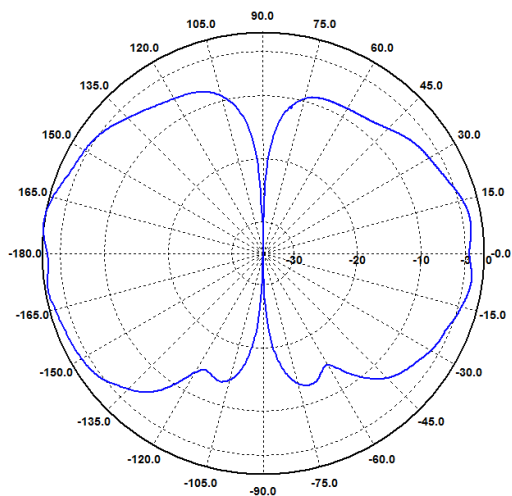
E-Ebene / E-Plane 3 GHz
