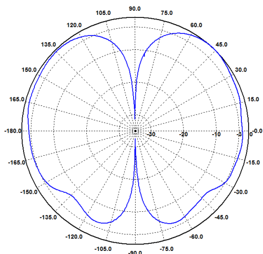
E-Ebene / E-Plane 2 GHz
