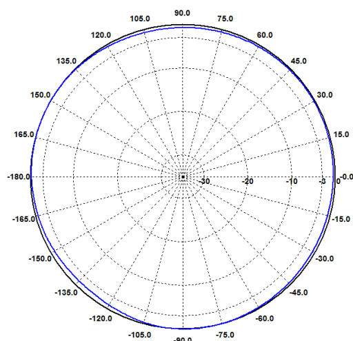
H-Ebene / H-Plane 1 GHz
